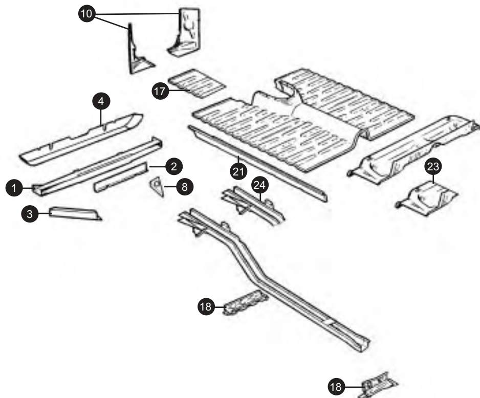
Underbody Panels
